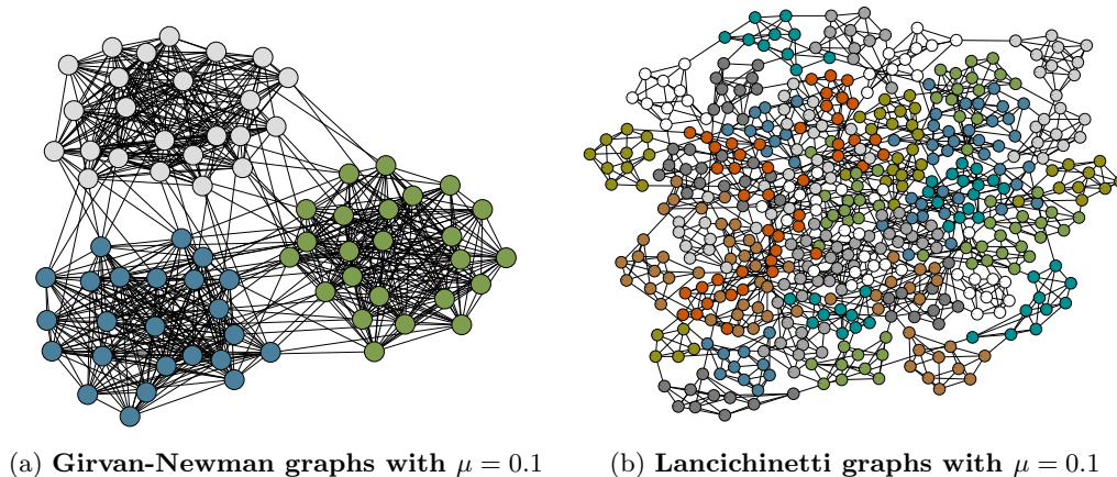
Figure 3: Benchmark graphs with planted partition
