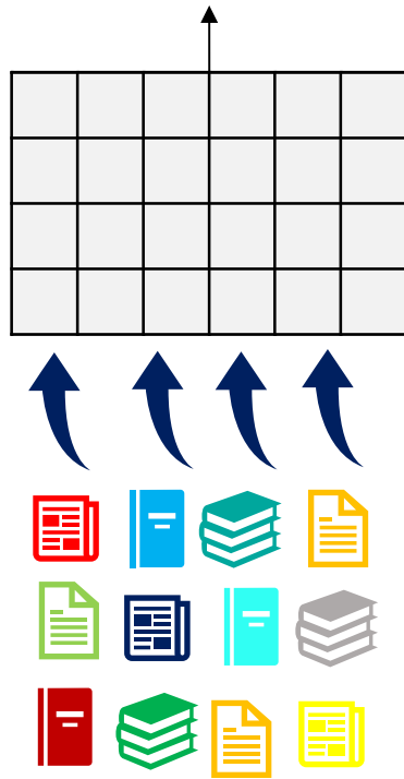
Pretraining
